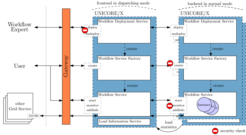
Fig. 2: BIS-Grid load balancing for UNICORE 6, backend nodes omitted
